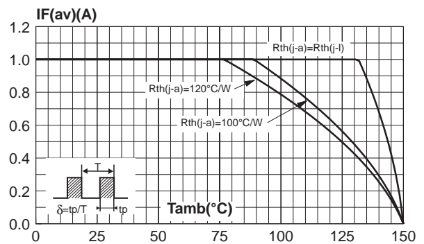
Fig. 2: Average forward current versus ambient temperature (δ=0.5).
